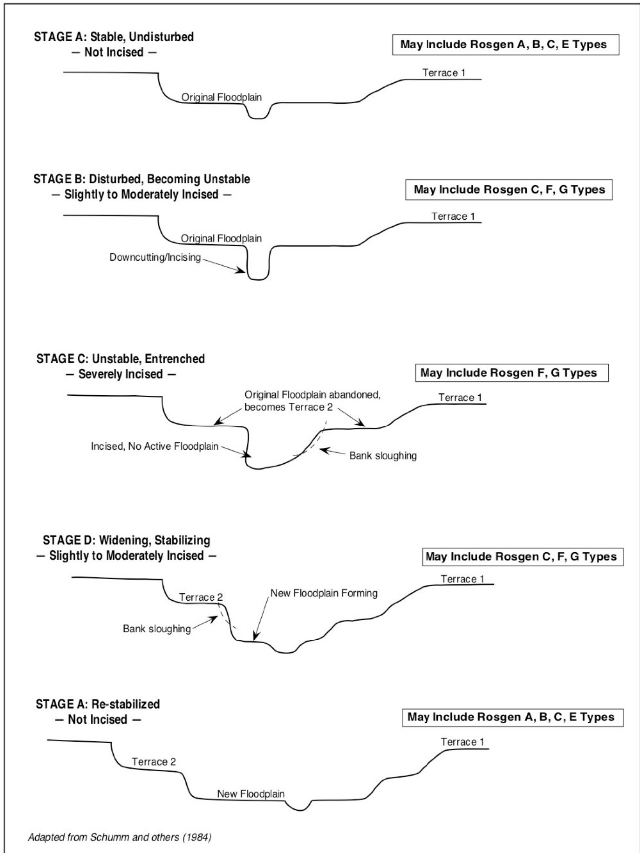
Figure 1. Schumm’s stages of stream channel evolution (Rosgen 2006), going from initial destabilization and incisement, through ultimate healing and re-stabilization with a new floodplain
